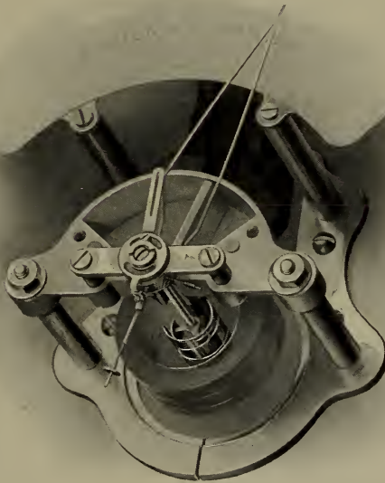
FIG. 26.—PHANTOM VIEW OF WESTON MODELS 151, 155, 156, 159, 160. Moving Parts of "Movable-Iron" Ammeters.
